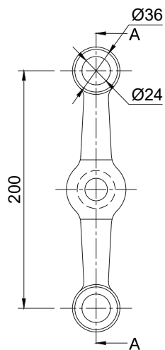
FRONT VIEW
